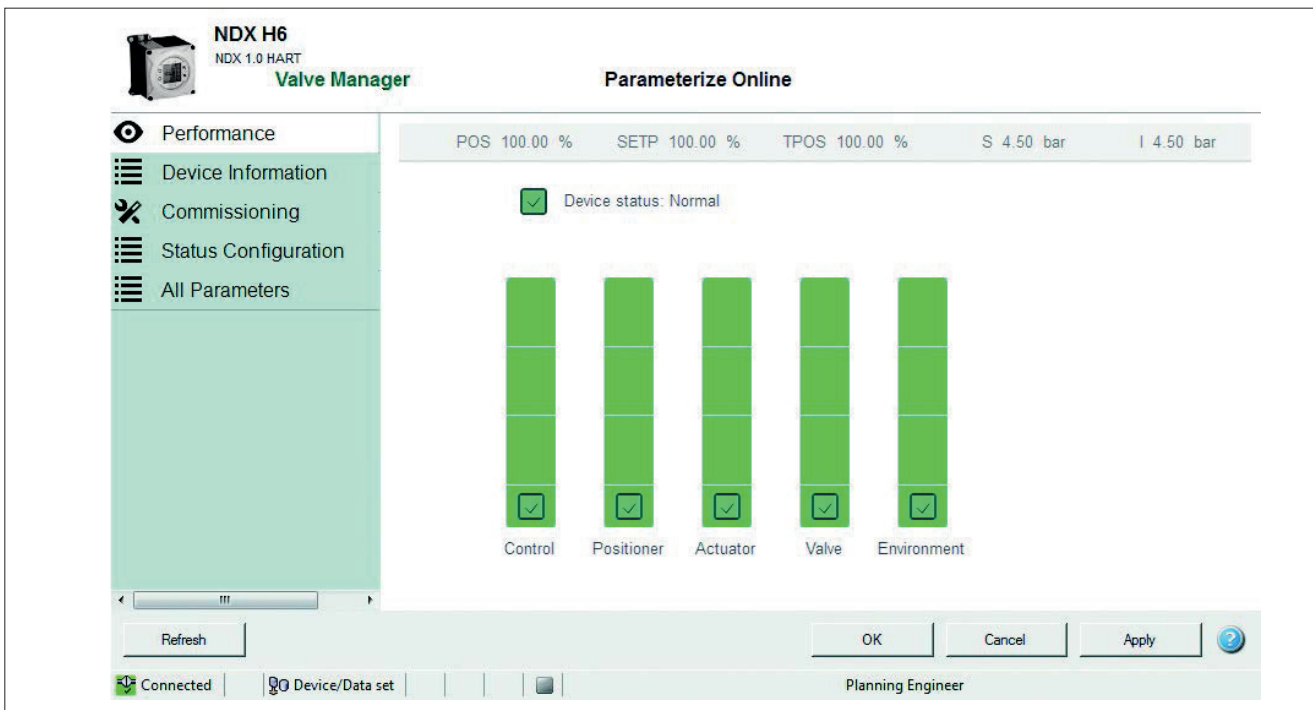
Fig. 2. The Performance View of the Neles Valve Manager graphically displays indexes of the valve, actuator and positioner, as well as indexes of control performance and the application environment. Report will show explanations of the status of each component and guidelines for recommended actions.
